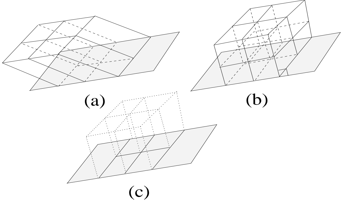
Fig. 18. (a) The 2-form D_1 - D_2 . (b) The 3-form n \wedge (D_1 - D_2) , with sides perpendicular to the boundary. (c) The 2-form \rho_s , represented by boxes on the boundary.
