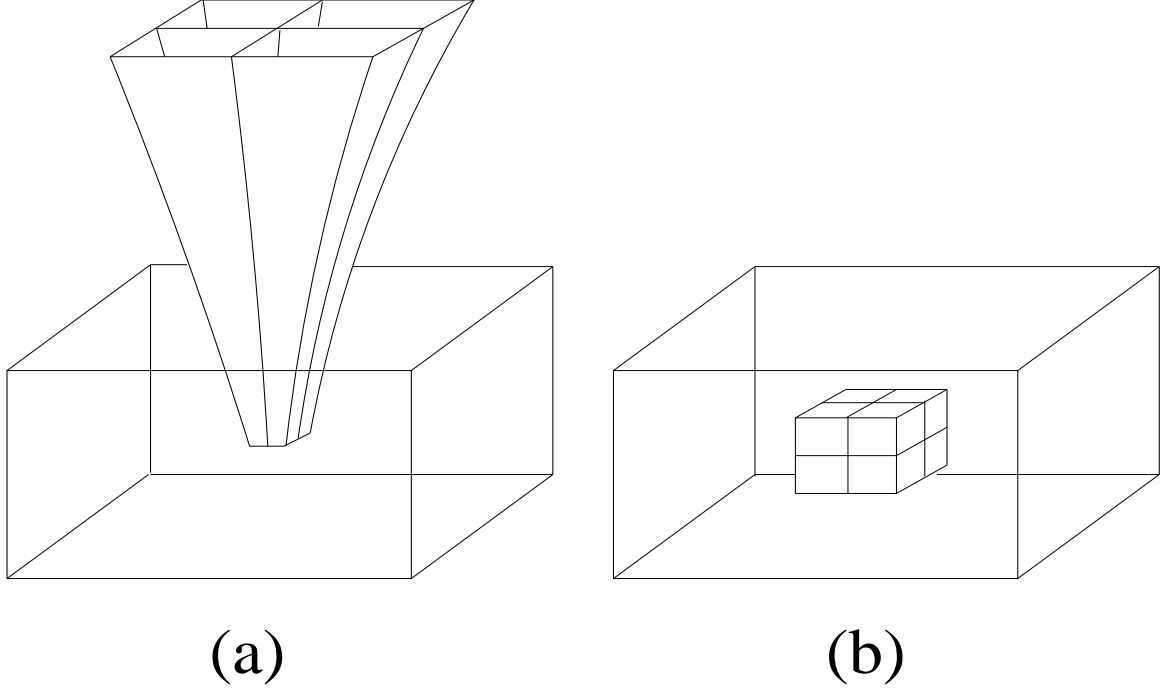
Fig. 16. Stokes theorem for \omega a 2-form. (a) Four tubes of the 2-form \omega pass through a surface. (b) The same number of boxes of the 3-form d\omega lie inside the surface.
