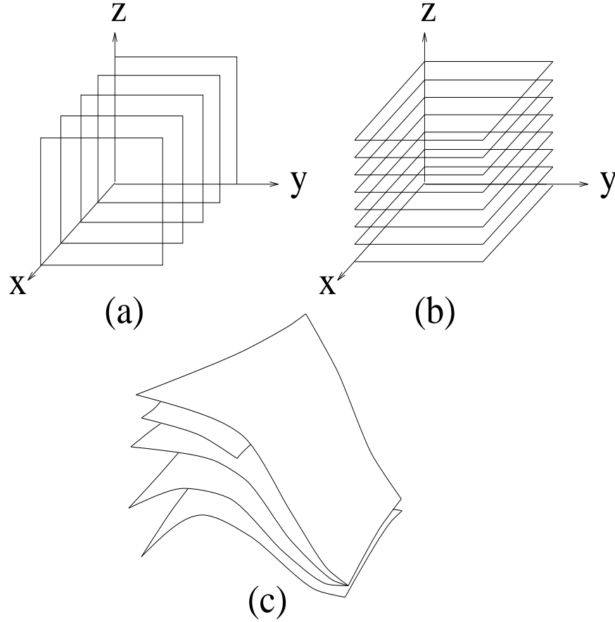
Fig. 1. (a) The 1-form dx , with surfaces perpendicular to the x axis and infinite in the y and z directions. (b) The 1-form dz , with surfaces perpendicular to the z -axis and spaced two per unit distance in the z direction. (c) A general 1-form, with curved surfaces and surfaces that end or meet each other.
