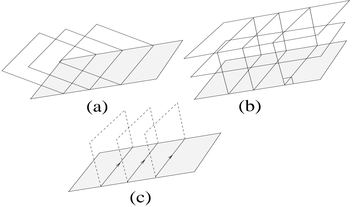
Fig. 17. (a) The 1-form H_1 - H_2 . (b) The 2-form n \wedge (H_1 - H_2) . (c) The 1-form J_s , represented by lines on the boundary. Current flows along the lines.
